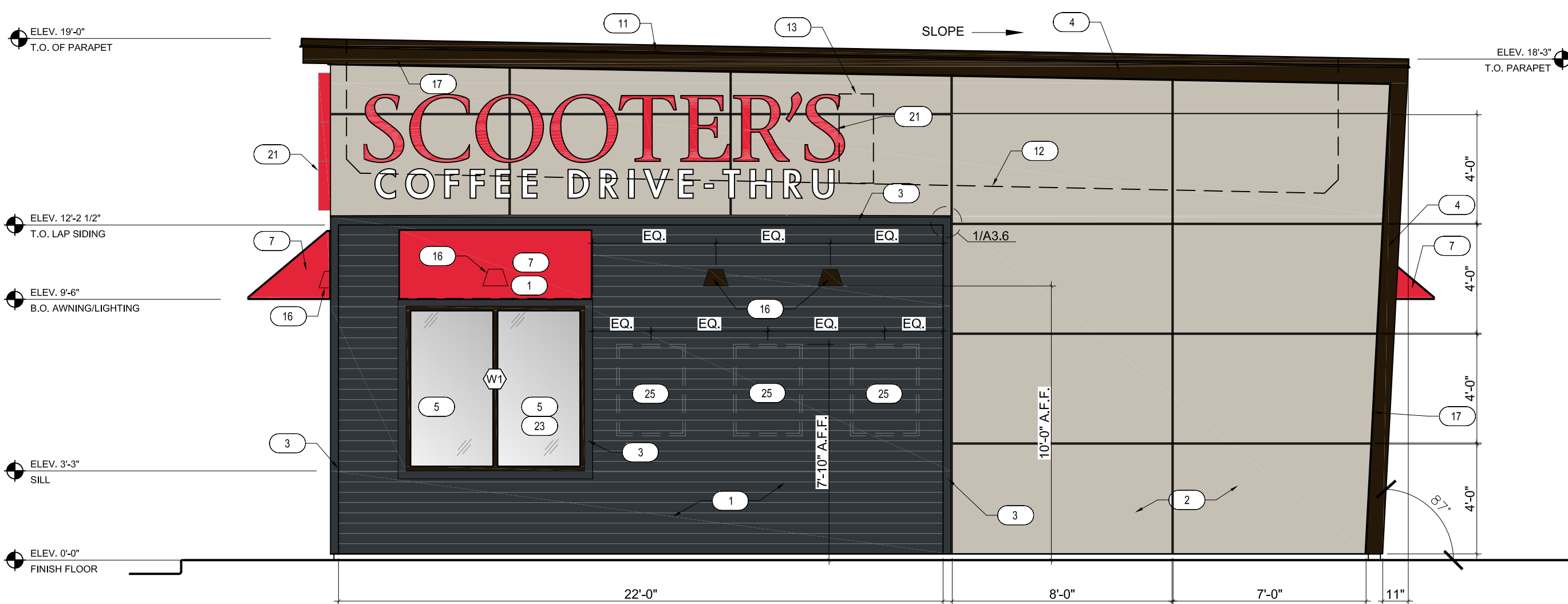
WEST ELEVATION
