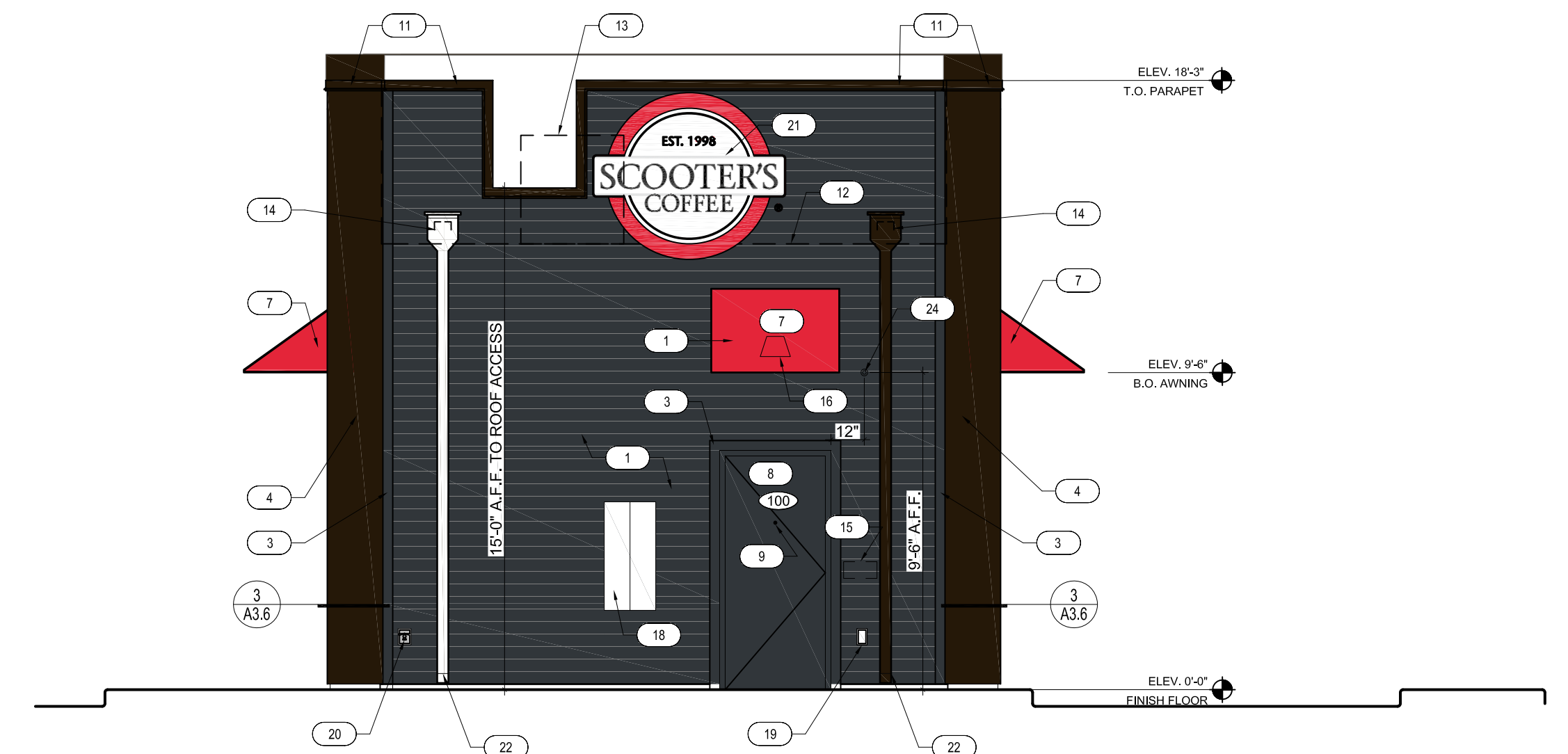
SOUTH ELEVATION
