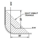
TYPICAL S.V.T. EASEMENT LOCAL TO LOCAL STREET N.T.S. (PER CITY OF SURREY ENGINEERING DESIGN STANDARD DETAIL 402)
